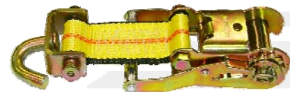
Part # 38-20SJ2 2" Wide Handle Ratchet with Web & Swivel J Hook WLL: 3,670 lbs
