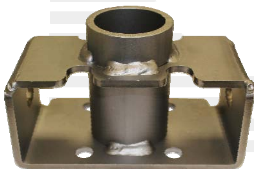
Part# XXXXX MOTOR MOUNT
